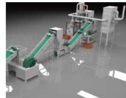
电路板/铜线/散热器/铝塑废弃物破碎分选设备 Circuit Board / Copper wire / Radiator / Aluminum plastic Waste Crushing and Separation Equipment
